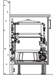
Typical installation STORMBOOST 60 (in cupboard)
