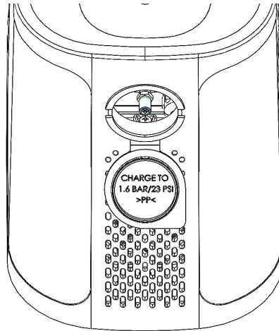
Figure 7 – Vessel Re-charging
