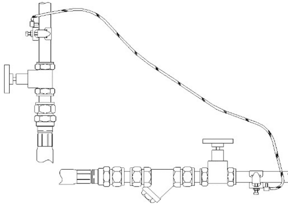
Figure 5 - Earth Continuity
