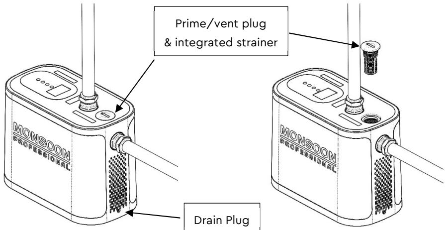
Figure 6 – Prime/vent/strainer and drain plug
