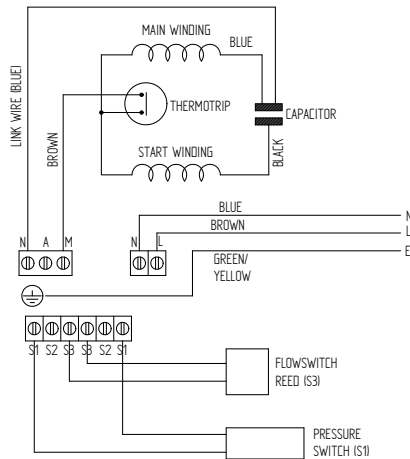
Monsoon Extra U1.4 bar Single Fig. 10
