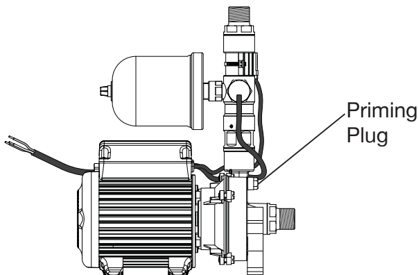
U1.4 bar Single Fig. 13
