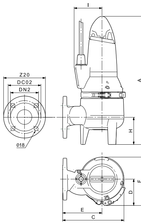
Fig. 48 Free-standing installation
