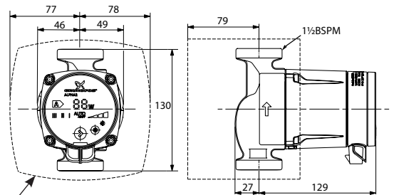
OPTIONAL INSULATION SHELL Part No:505821
